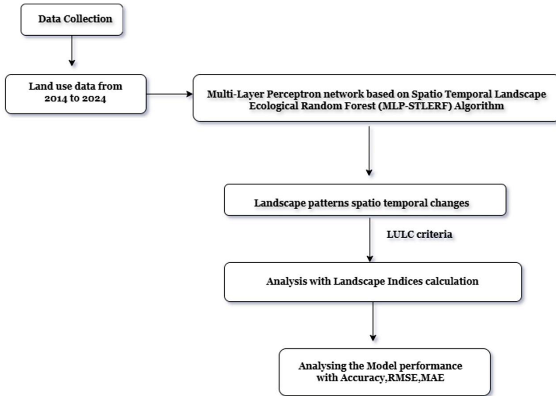
Figure 1. Flowchart of proposed MLP-STLERF algorithm.
