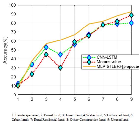
Figure 5. Outcome of accuracies of compared models.
